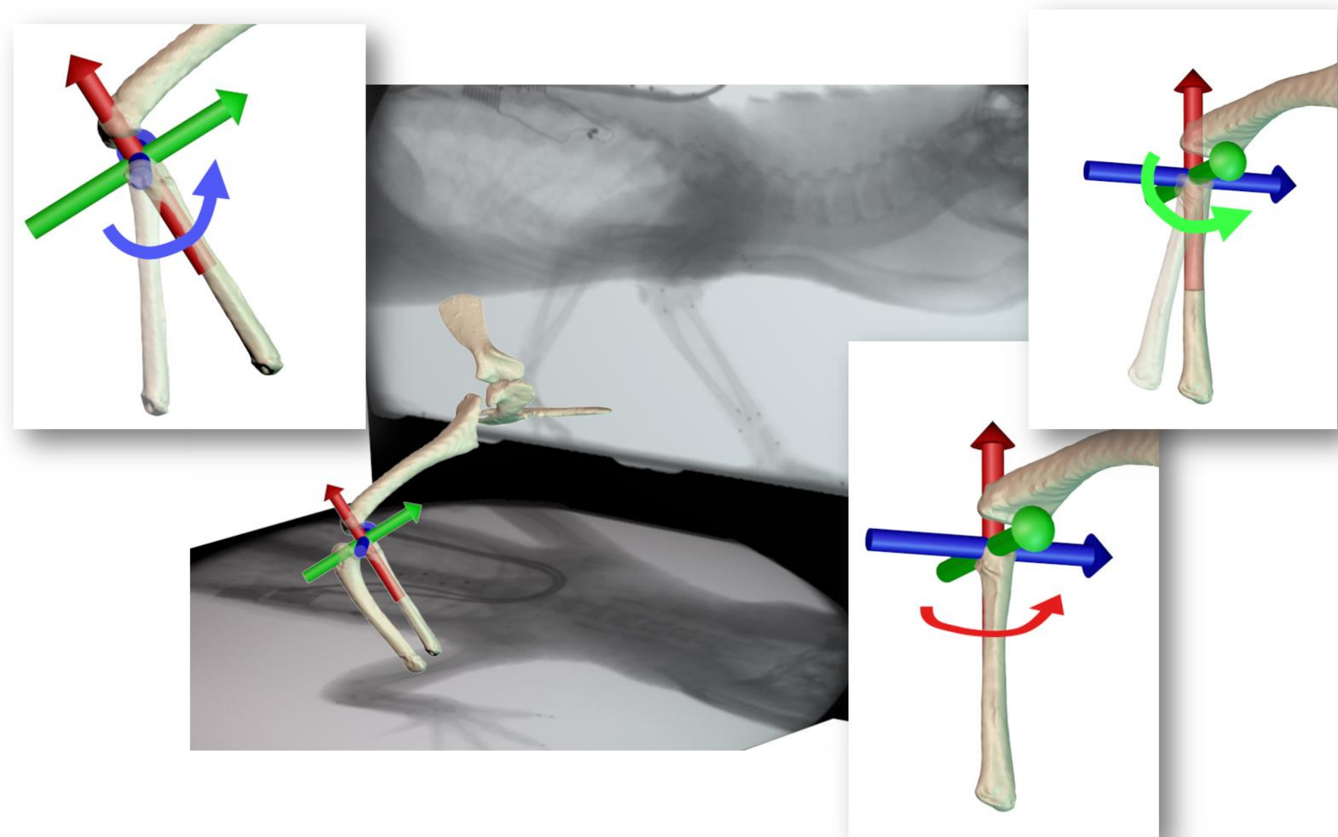
Figure 2. Alligator bone model aligned with 2 cameras X-ray imaging. In the bone models, the red arrow is showing the x-axis of rotation (long axis). The green arrow is showing the y-axis rotation (abduction/adduction). The blue arrow is showing the x-axis of rotation (flexion/extension).
